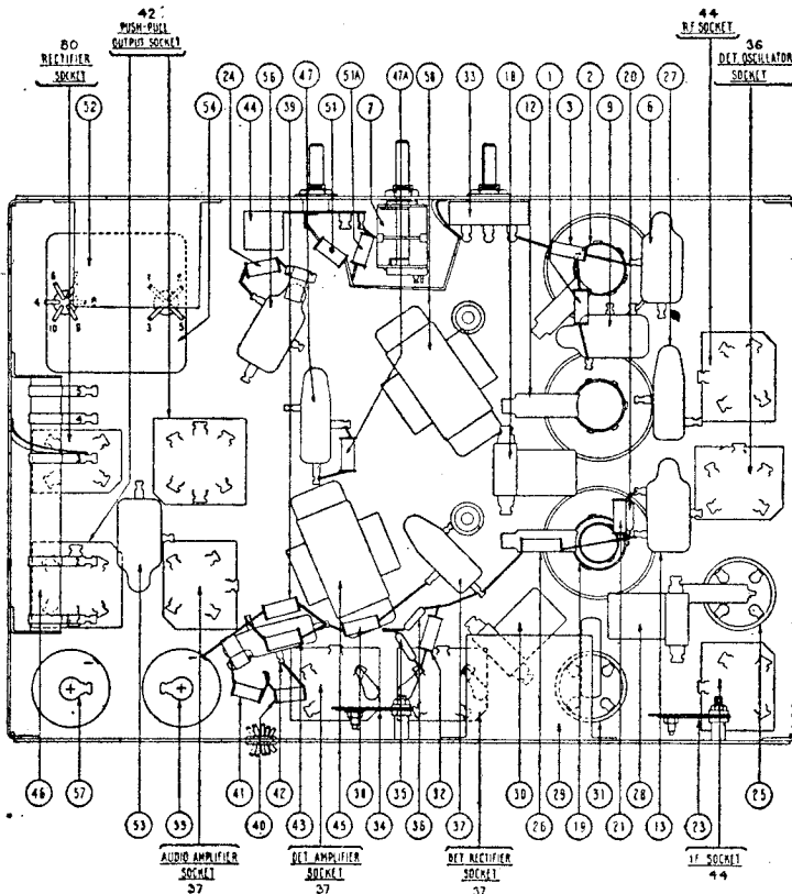
Fig. 1—Parts Diagram
